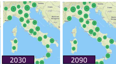
Wildfires
