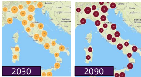
Water Stress
