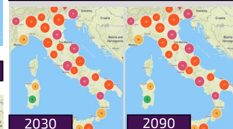
Earthquakes
